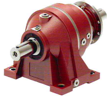
AXIAL PLANETARY GEARBOX WITH FEET AND DOUBLE INPUT OUTPUT FLANGE
