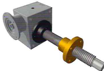
SERIES CHS10 TS or RS - load kg 40.000
