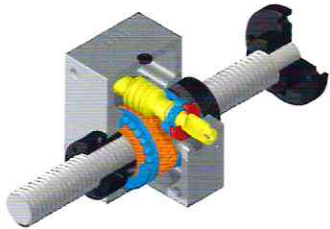
SERIES CHS3 TS or RS - load kg 2.500
